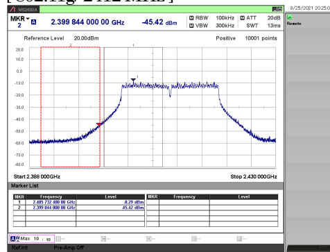
[ 802.11g/ 2412 MHz ]
