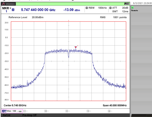
[ 802.11a/ 5745 MHz ]
