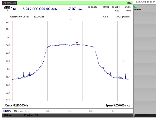
[ 802.11a/ 5240 MHz ]
