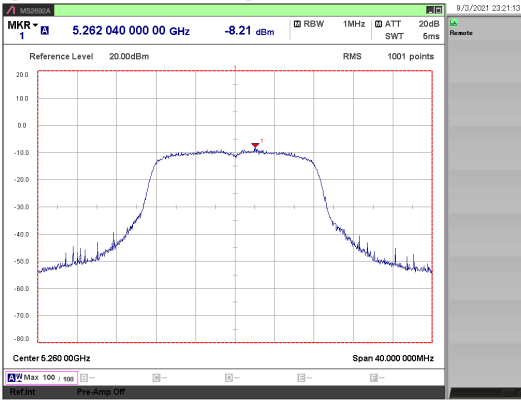
[ 802.11a/ 5260 MHz ]
