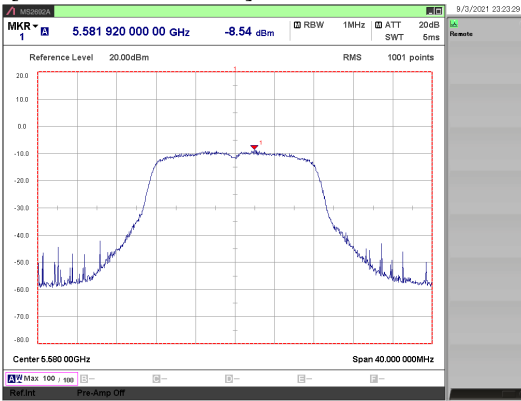
[ 802.11a/ 5580 MHz ]
