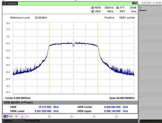
[ 802.11a/ 5300 MHz ]
