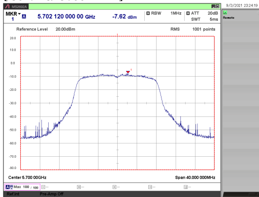
[ 802.11a/ 5700 MHz ]
