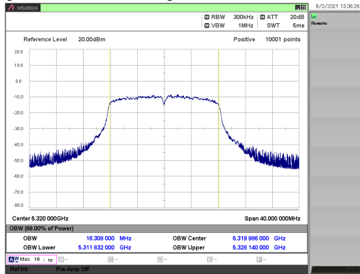
[ 802.11a/ 5320 MHz ]
