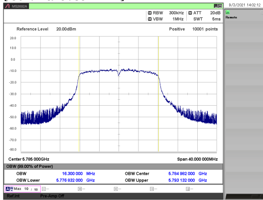
[ 802.11a/ 5785 MHz ]
