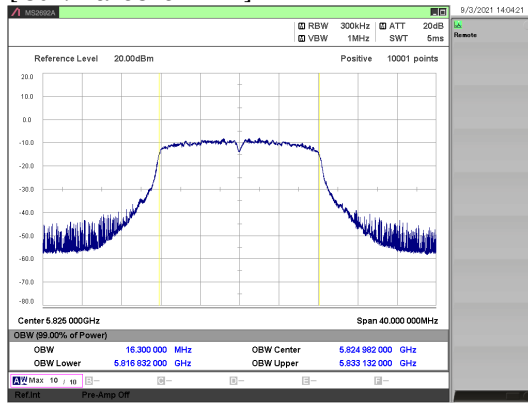
[ 802.11a/ 5825 MHz ]
