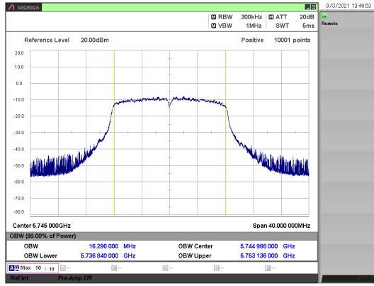
[ 802.11a/ 5745 MHz ]
