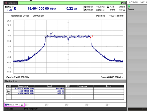
[ 802.11g/ 2462 MHz ]
