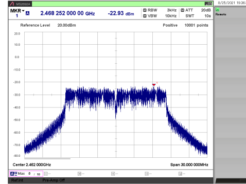
[ 802.11g/ 2462 MHz ]
