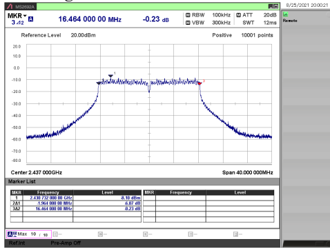
[ 802.11g/ 2437 MHz ]
