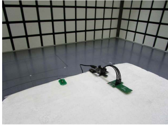
Antenna X-axis
