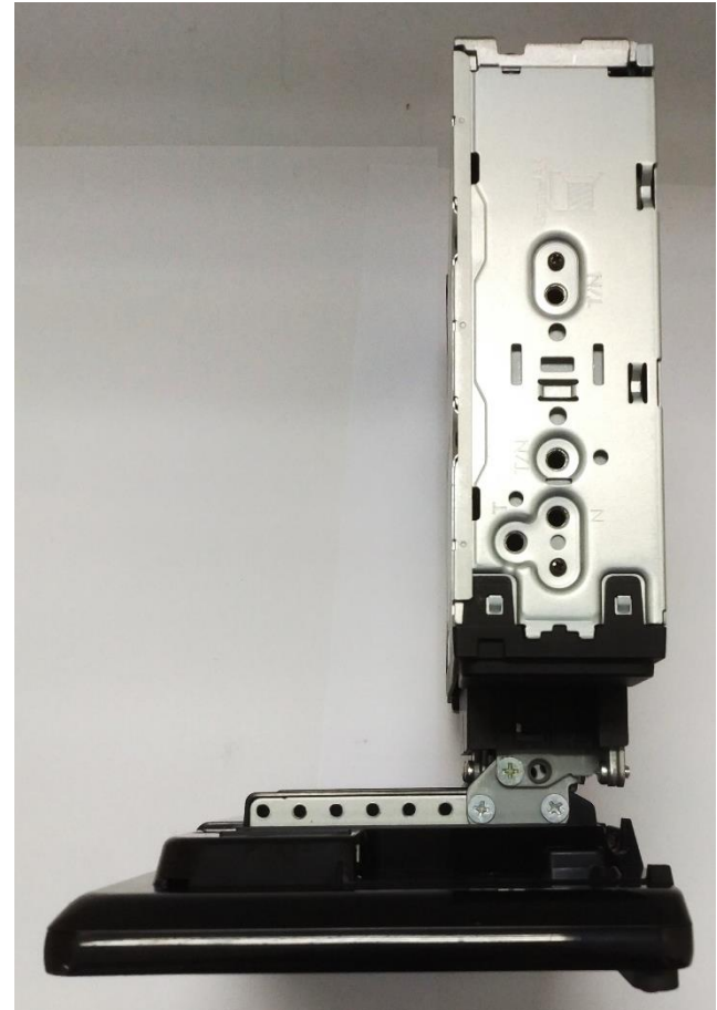
RIGHT SIDE
