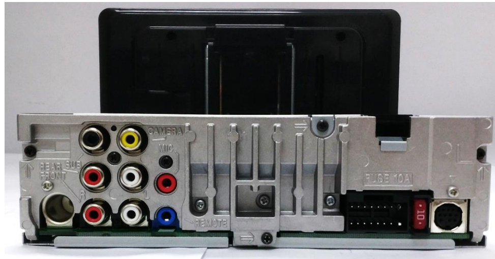
BACK SIDE
