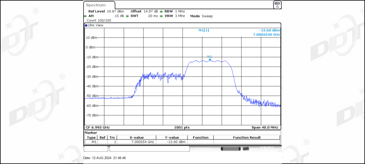
11AX20MIMO Ant-3 6995 26Tone RU0
