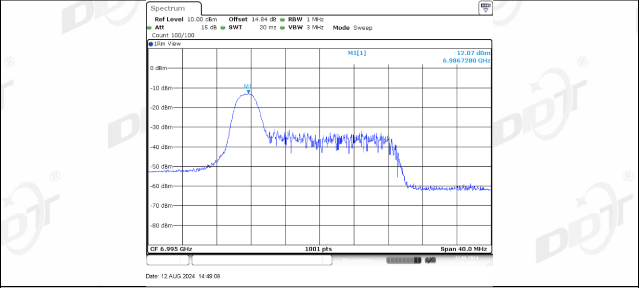
11AX20MIMO Ant-3 6995 26Tone RU4
