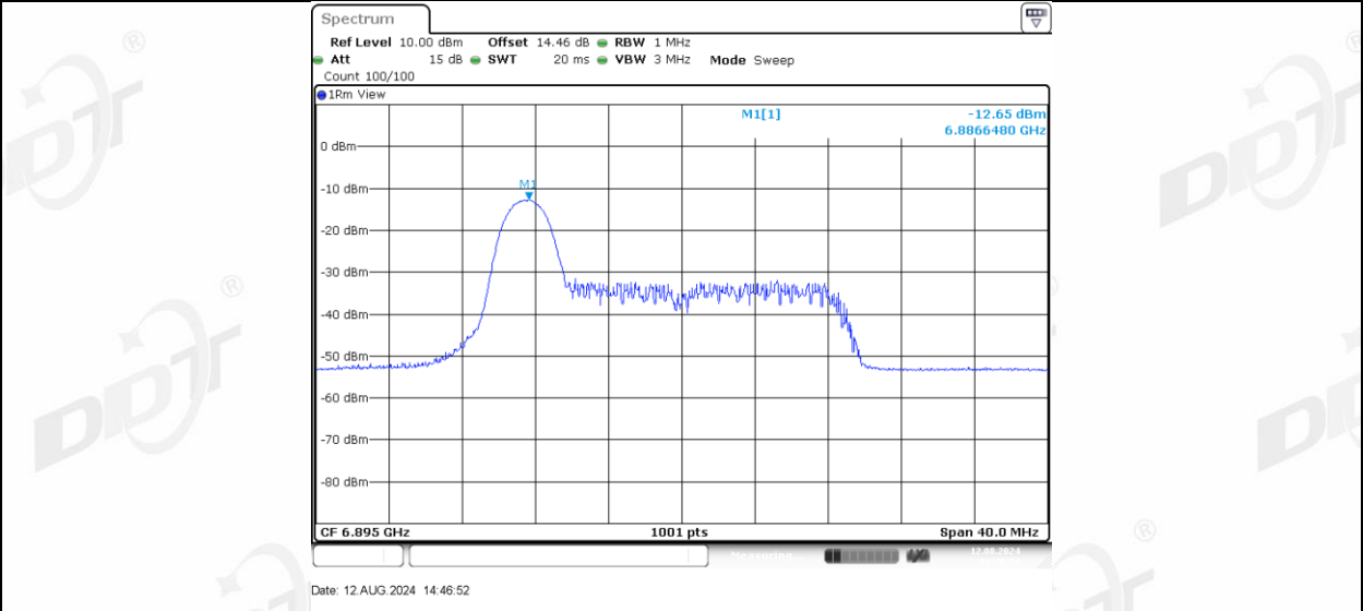
11AX20MIMO Ant-3_6895_26Tone_RU4
