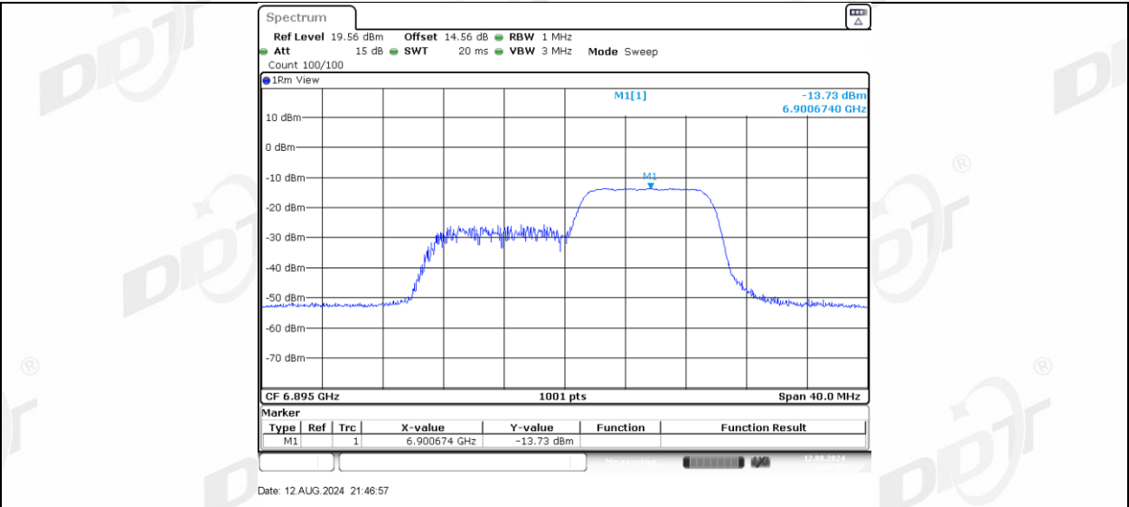
11AX20MIMO Ant-3_6895_26Tone_RU0
