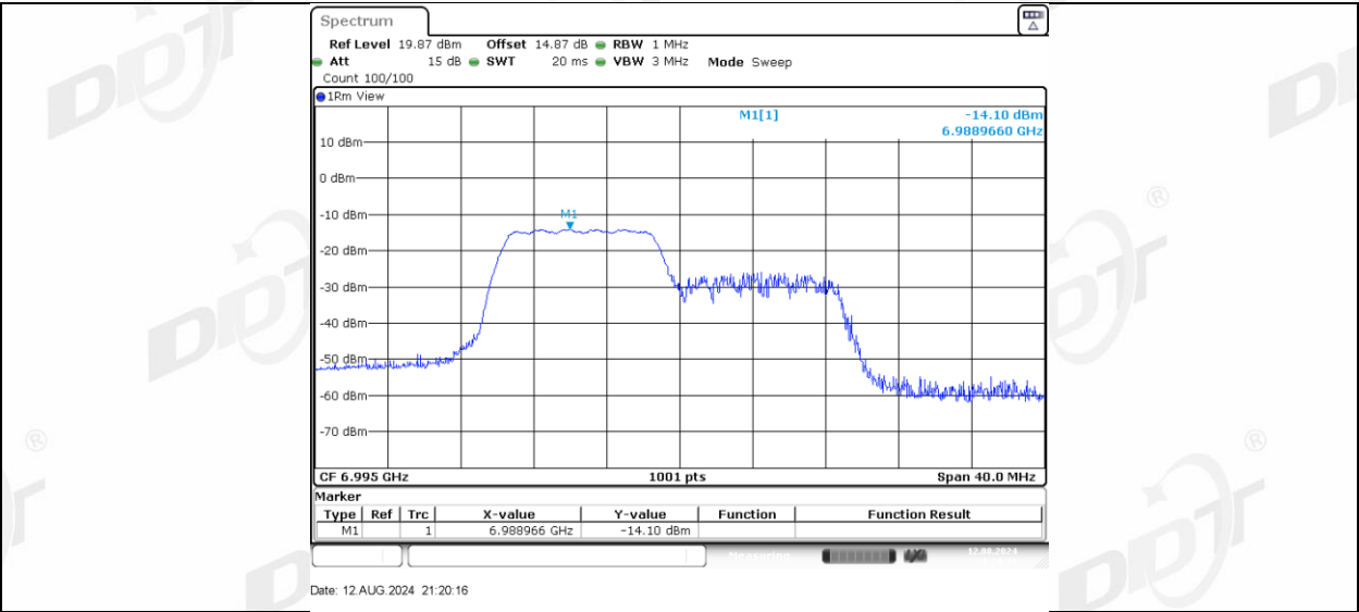
11AX20MIMO Ant-1 6995 106Tone RU54
