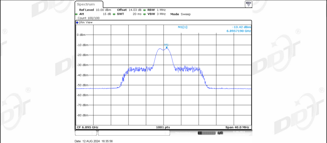
11AX20MIMO Ant-3_6895_26Tone_RU8
