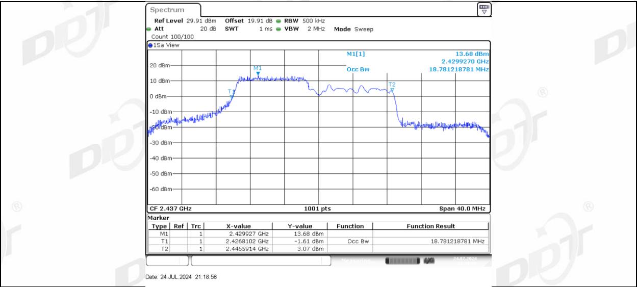
11AX20MIMO Ant-3_2437_106Tone_RU54
