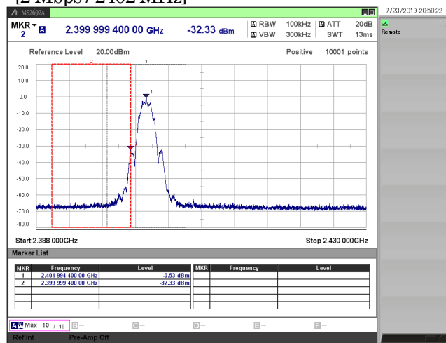
[2 Mbps / 2402 MHz]
