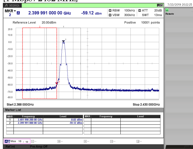
[1 Mbps / 2402 MHz]
