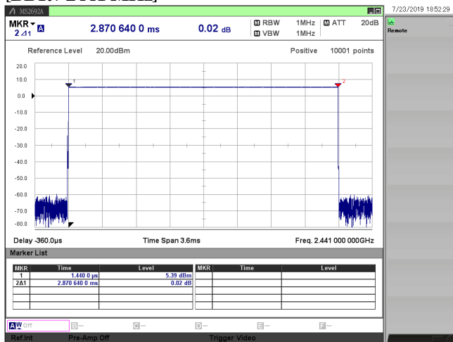
[BDR / 2441 MHz]
