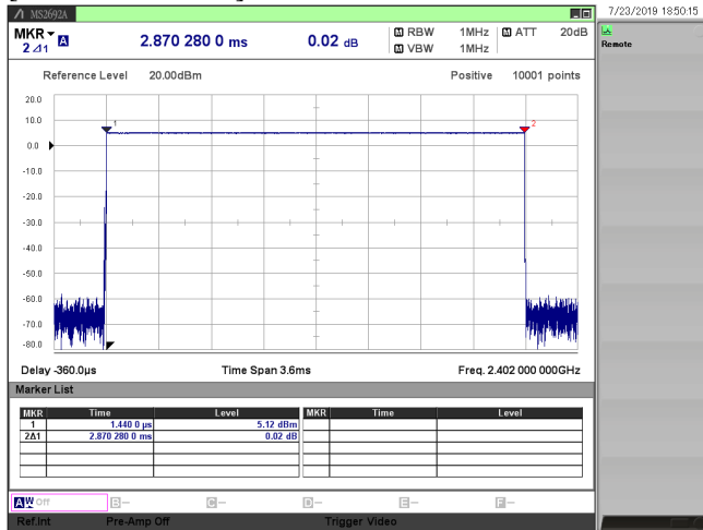
[BDR / 2402 MHz]
