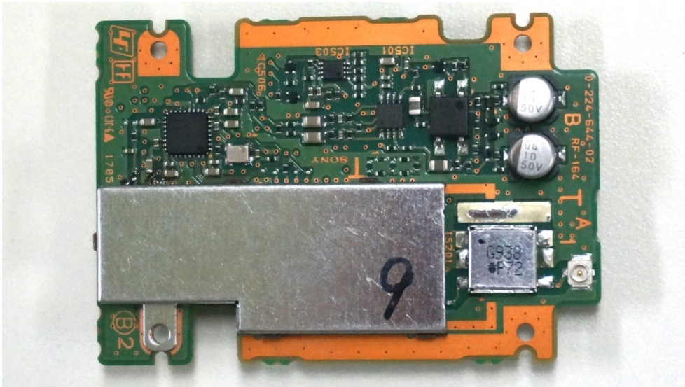
Fig.7: Side B of board RF-164 with shield case
