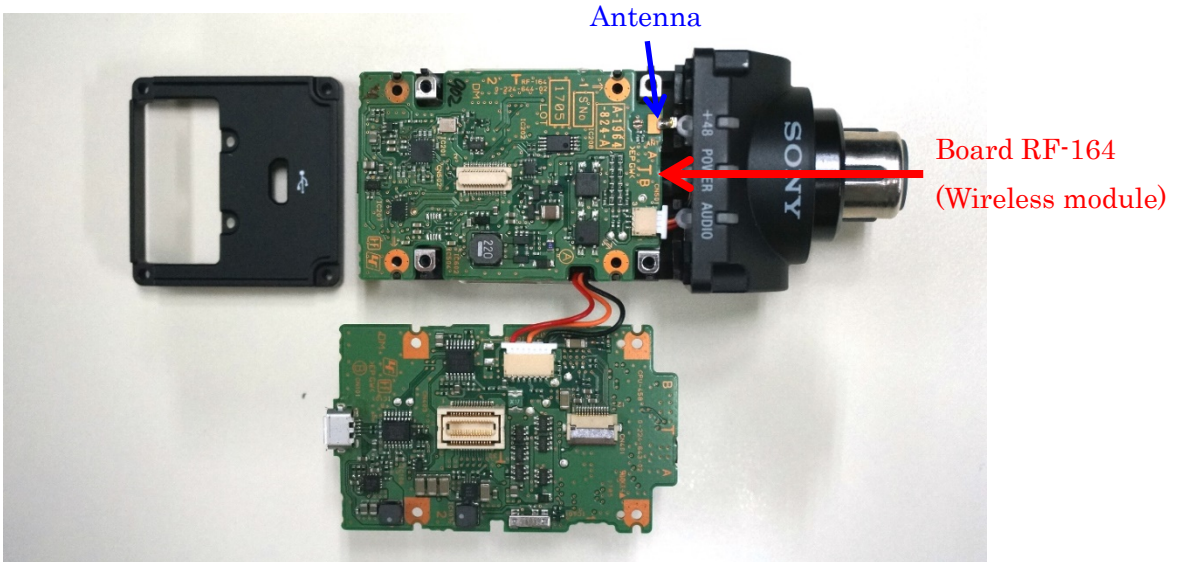
Fig.2: Removed the upper board (Place of board RF-164)
