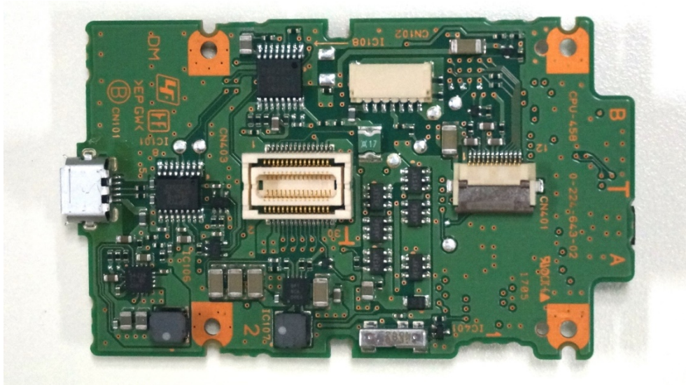
Fig.4: Side B of board CPU-458
