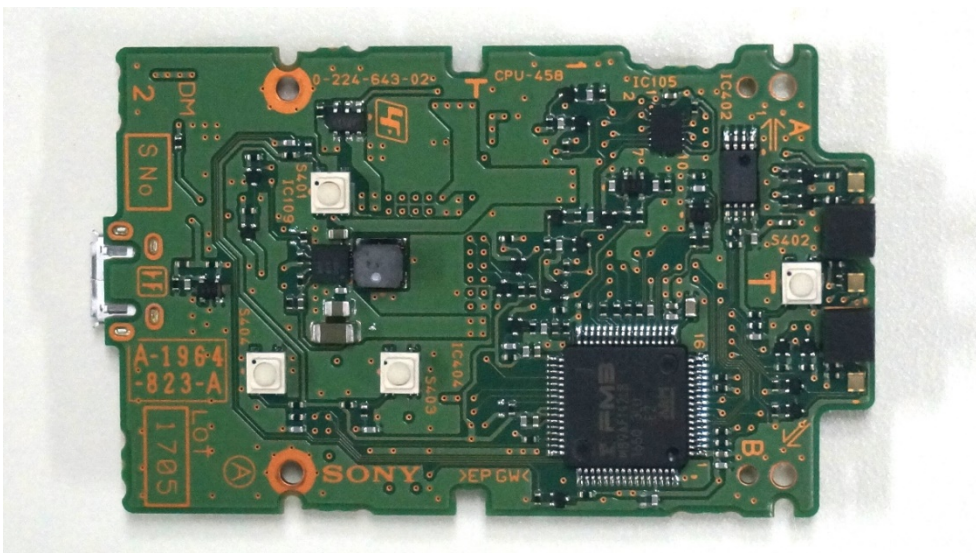
Fig.3: Side A of board CPU-458
