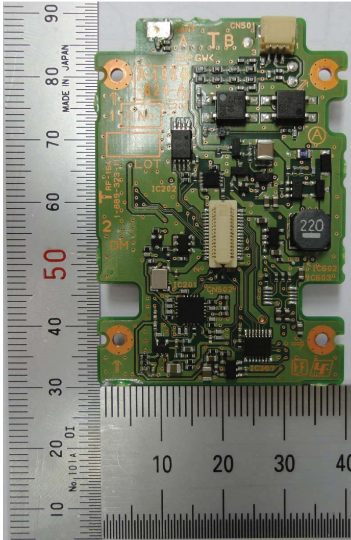
Side A of Board RF-164
