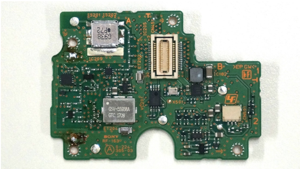
Fig.5: Side A of board RF-163
