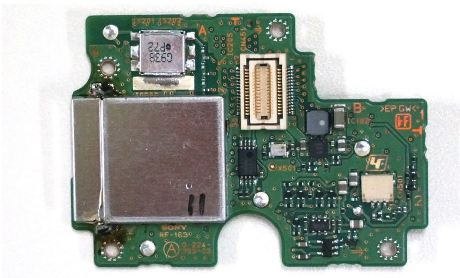
Fig.6: Side A of board RF-163 with shield case
