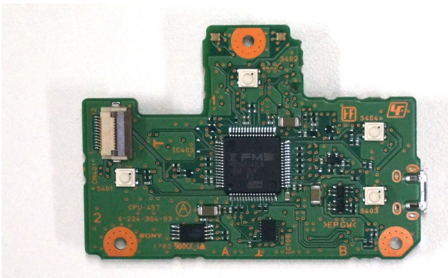
Fig.3: Side A of board CPU-457
