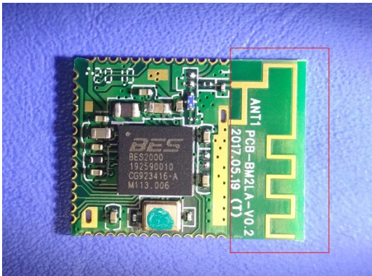
Module/antenna photo
