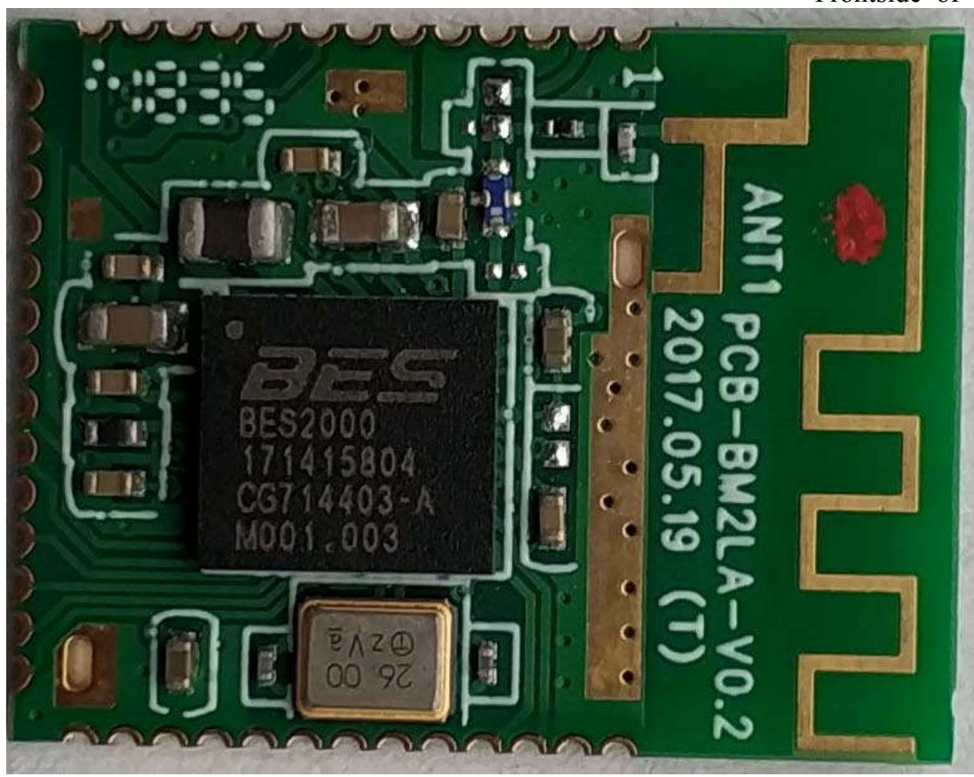
Figure 16 Frontside of RF Module
