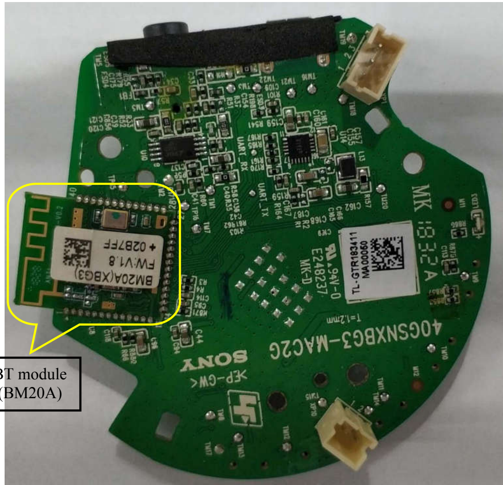
Figure 16 Frontside of RF Module
