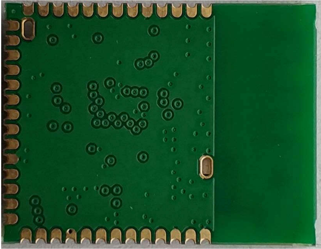
Figure 17 Backside of RF Module
