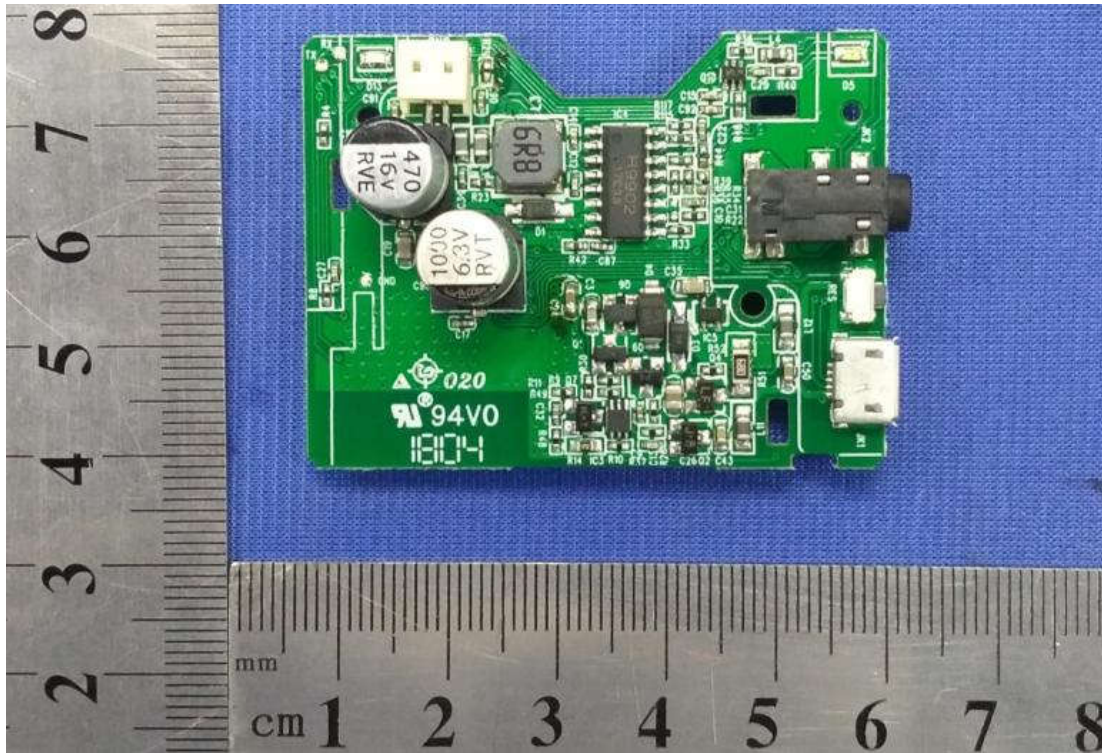
Figure 7 PCB Bottom of the EUT
