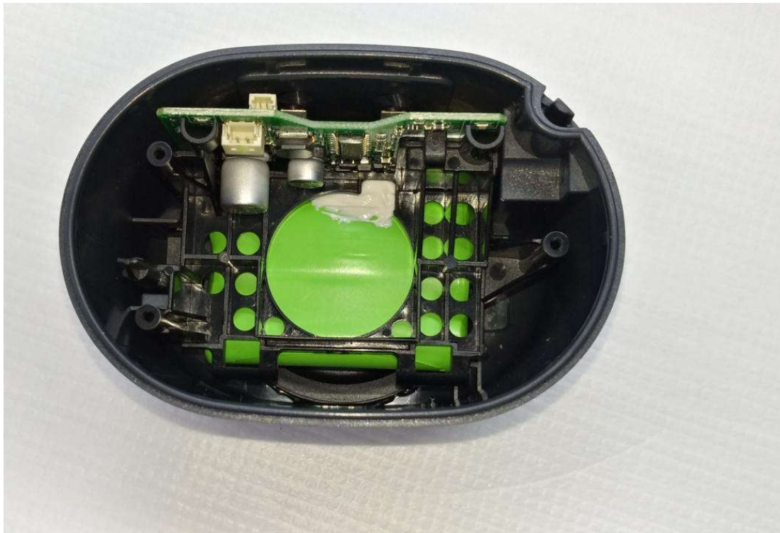
Figure 2 Rear with PCB of the EUT
