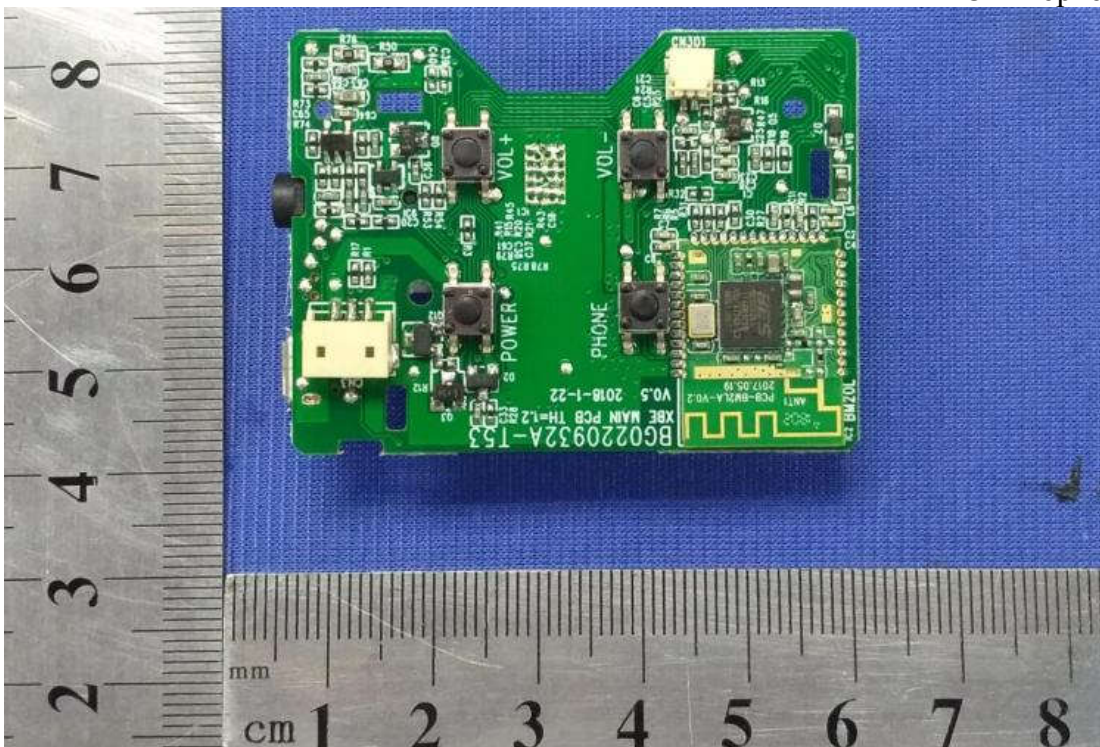
Figure 6 PCB Top of the EUT
