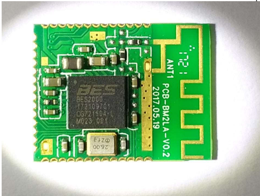
Figure 10 Module Top of the EUT
