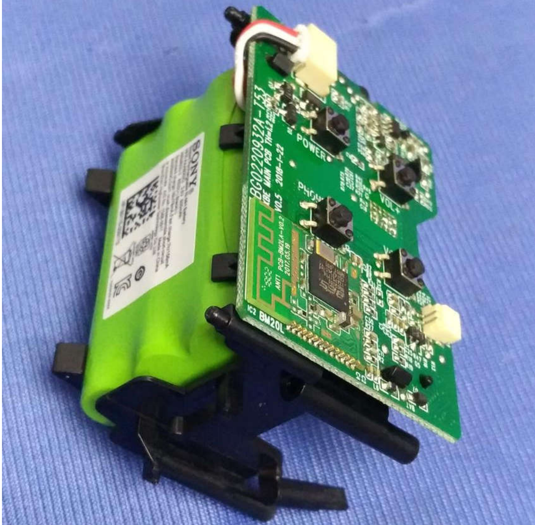
Figure 6 PCB Top of the EUT
