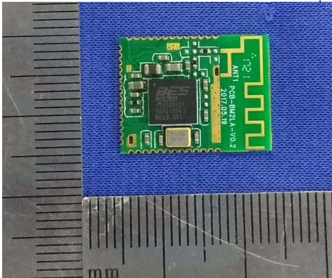
Figure 8 BTM Top of the EUT
