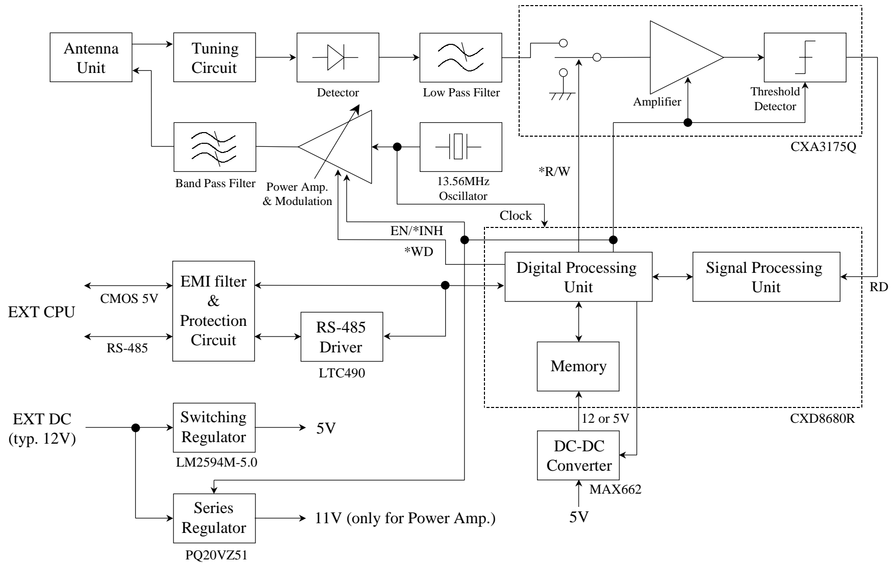
Block Diagram of RC-S430C
