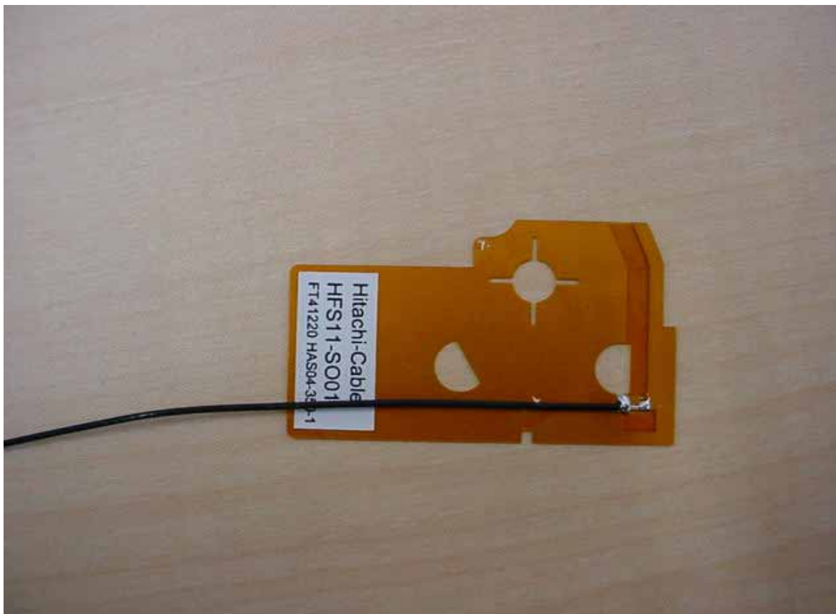
Photo 15 Antenna - b
