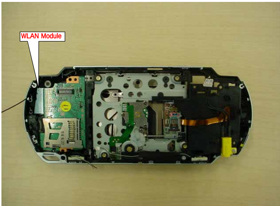
Photo 4 Inside(5/5) / Location of WLAN Module
