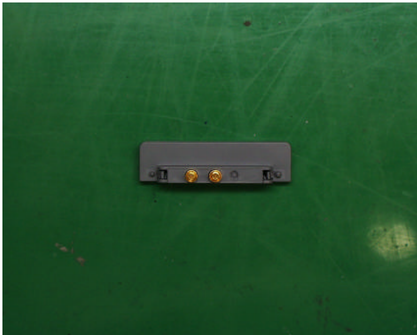
Antenna (Back)
