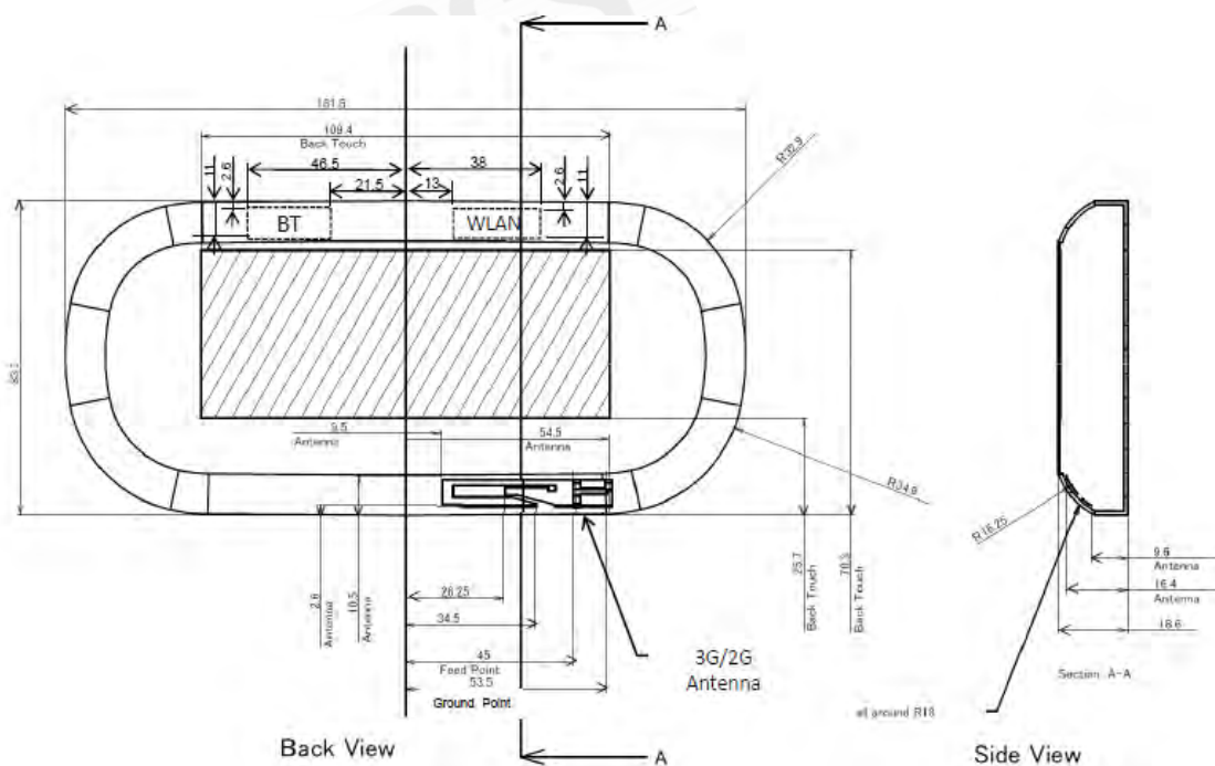
Fig.11 Antenna position of EUT
