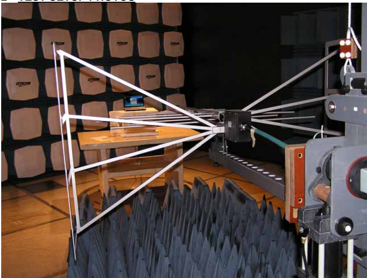
RADIATED EMISSIONS
