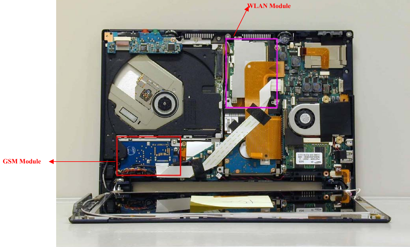
Laptop Internal view showing location of WLAN and GSM modules
