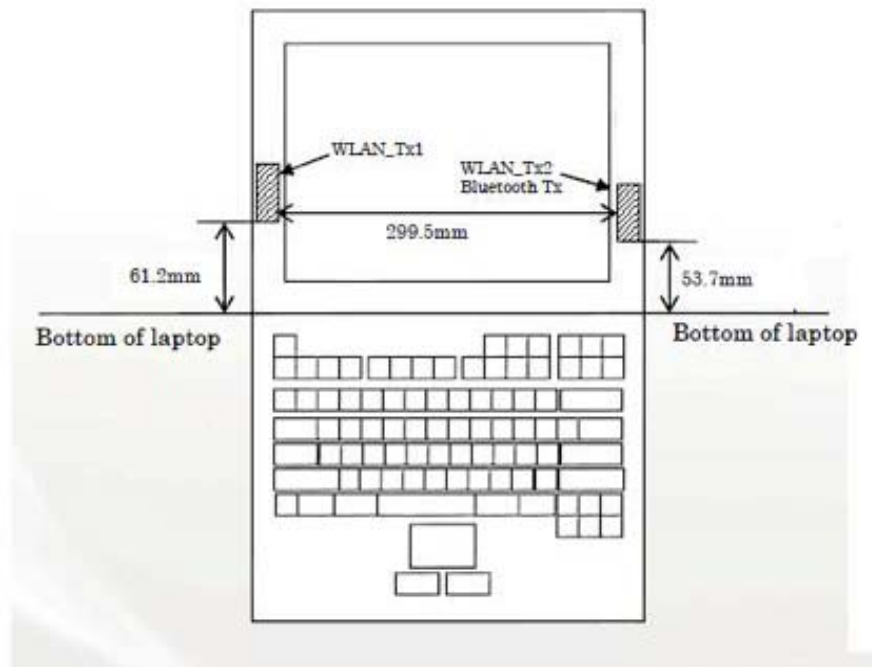
Figure 10-2 Antenna Diagram
