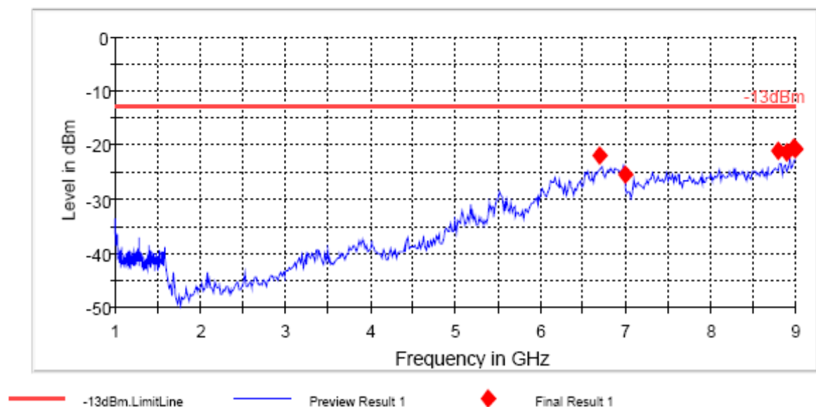
FCC 22 1-9GHz
