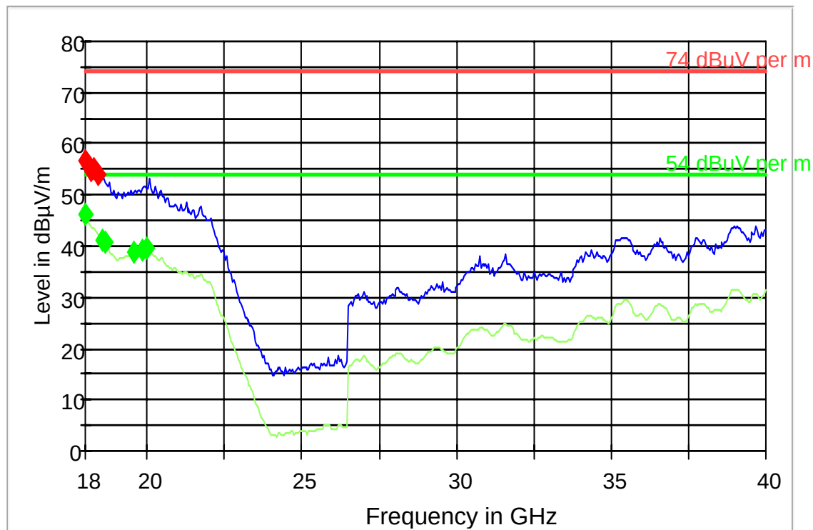
FCC 15 18-40GHz
