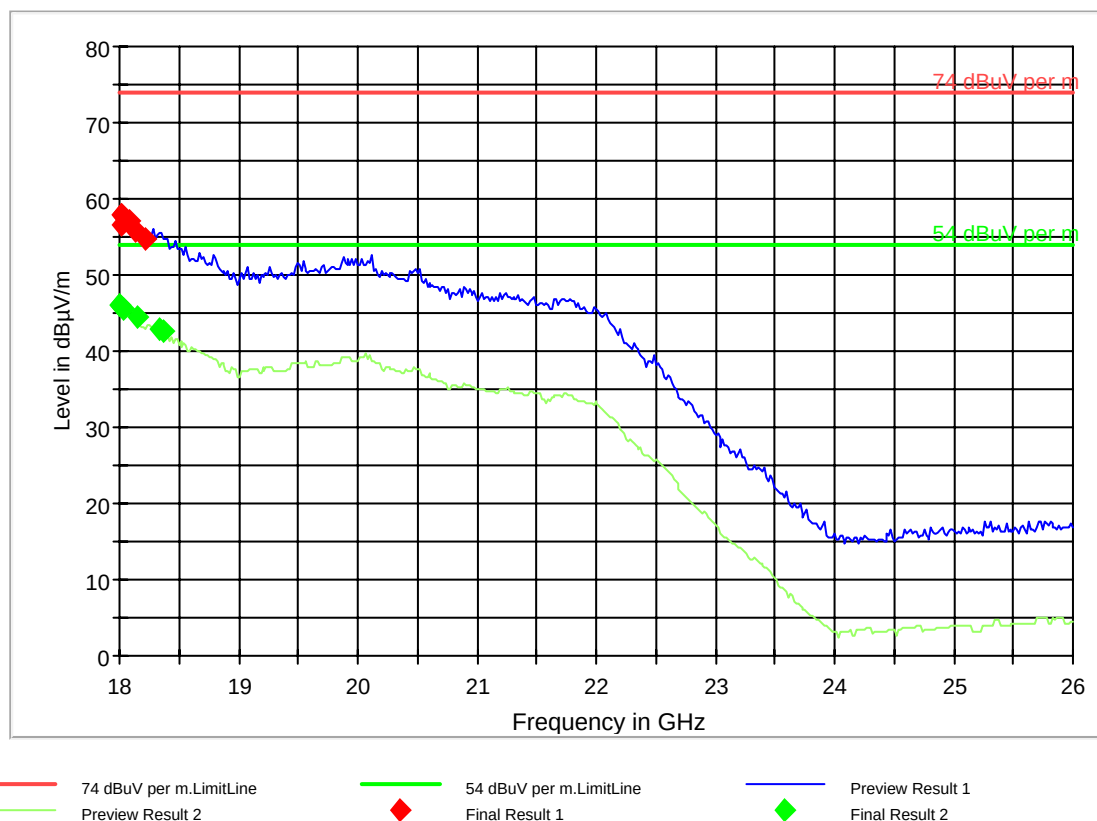
FCC 15 18-26GHz
