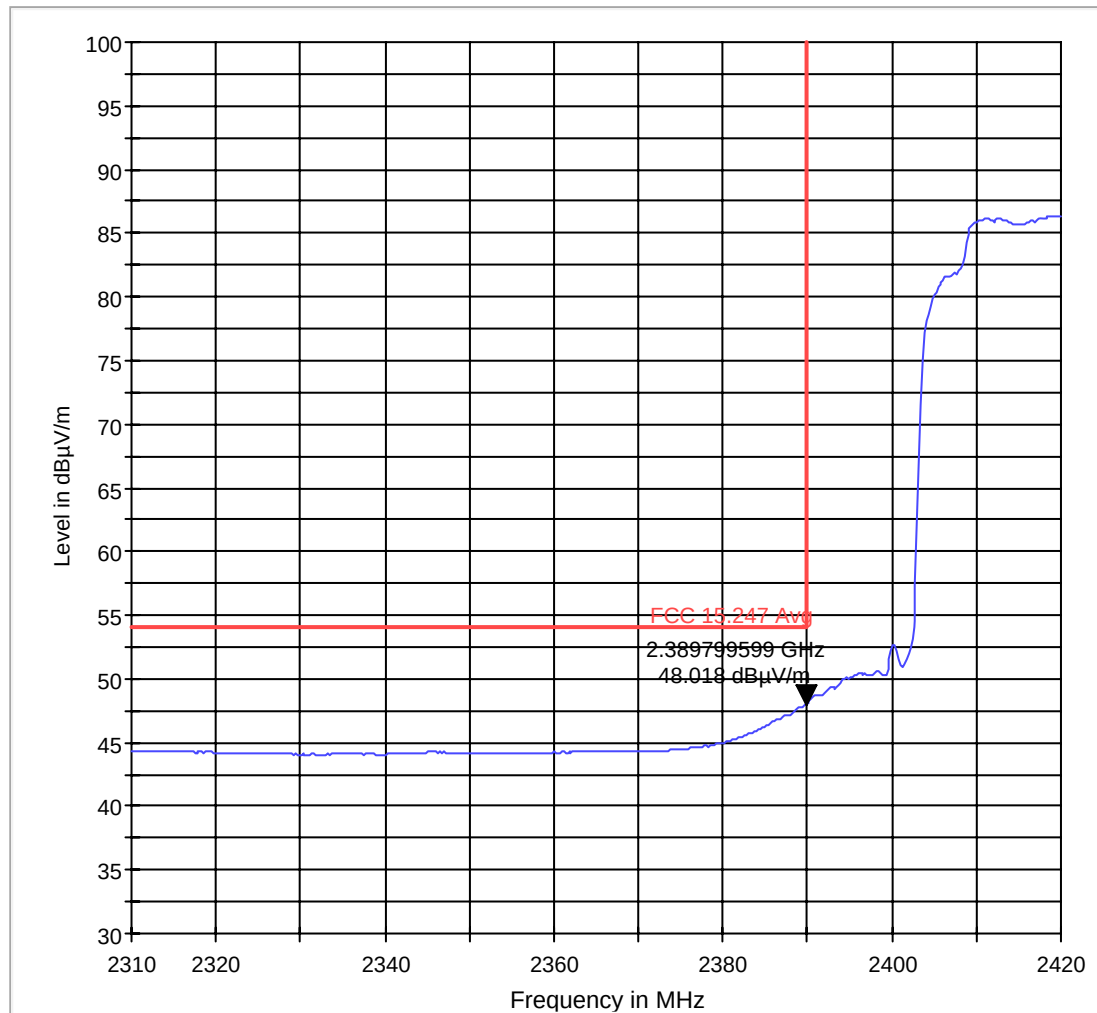
FCC 15.247 LBE Avg 3m
