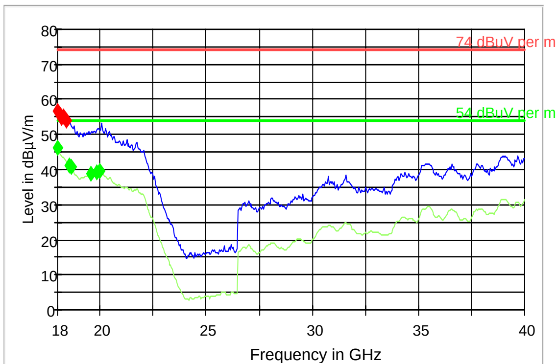
FCC 15 18-40GHz
