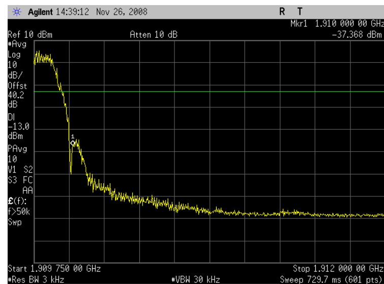
Plot 6.2 - 8 (Ch810, 8PSK)
