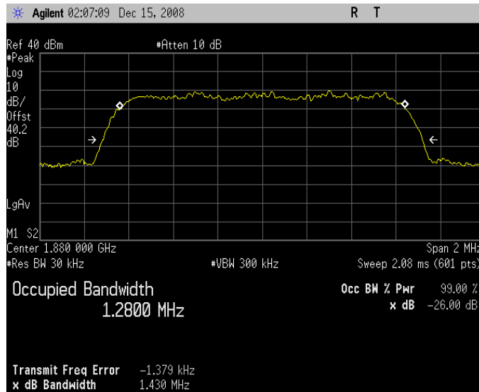
Plot 5.2 - 41 (Ch600, Rel A, 4096 payload size)
