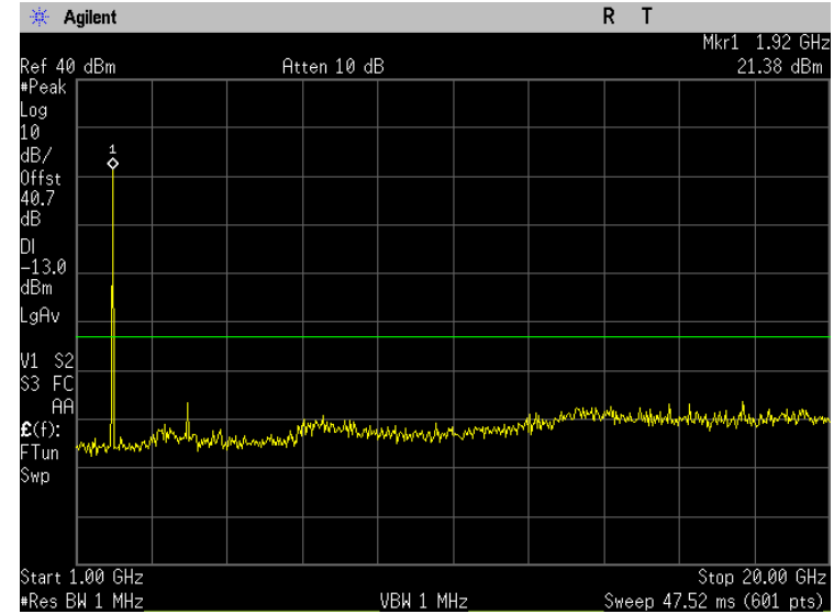
Plot 7.2 - 36 (WCDMA, Rel99, Ch9538)
