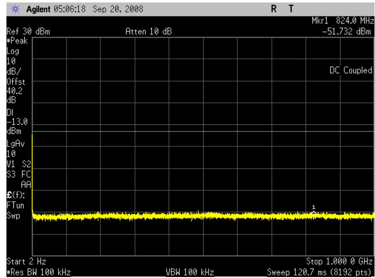
Plot 7.2 - 35 (WCDMA, Rel99, Ch9538)
