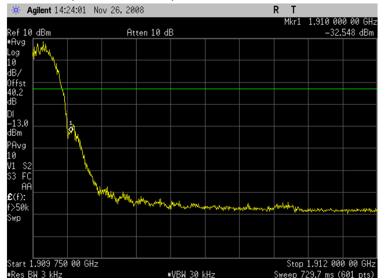
Plot 6.2 - 4 (Ch810, GSM1900)
