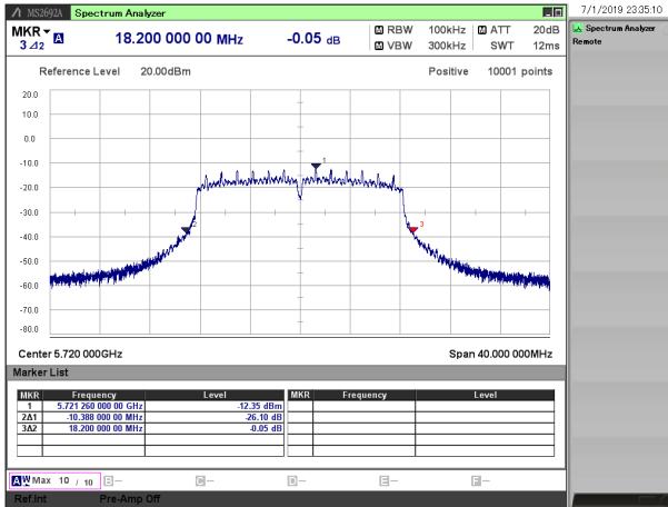
[ 802.11a/ 5720 MHz ]
