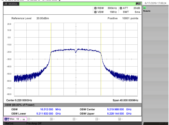
[ 802.11a/ 5220 MHz ]
