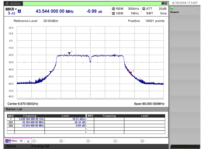
[ 802.11ac (VHT40)/ 5670 MHz ]
