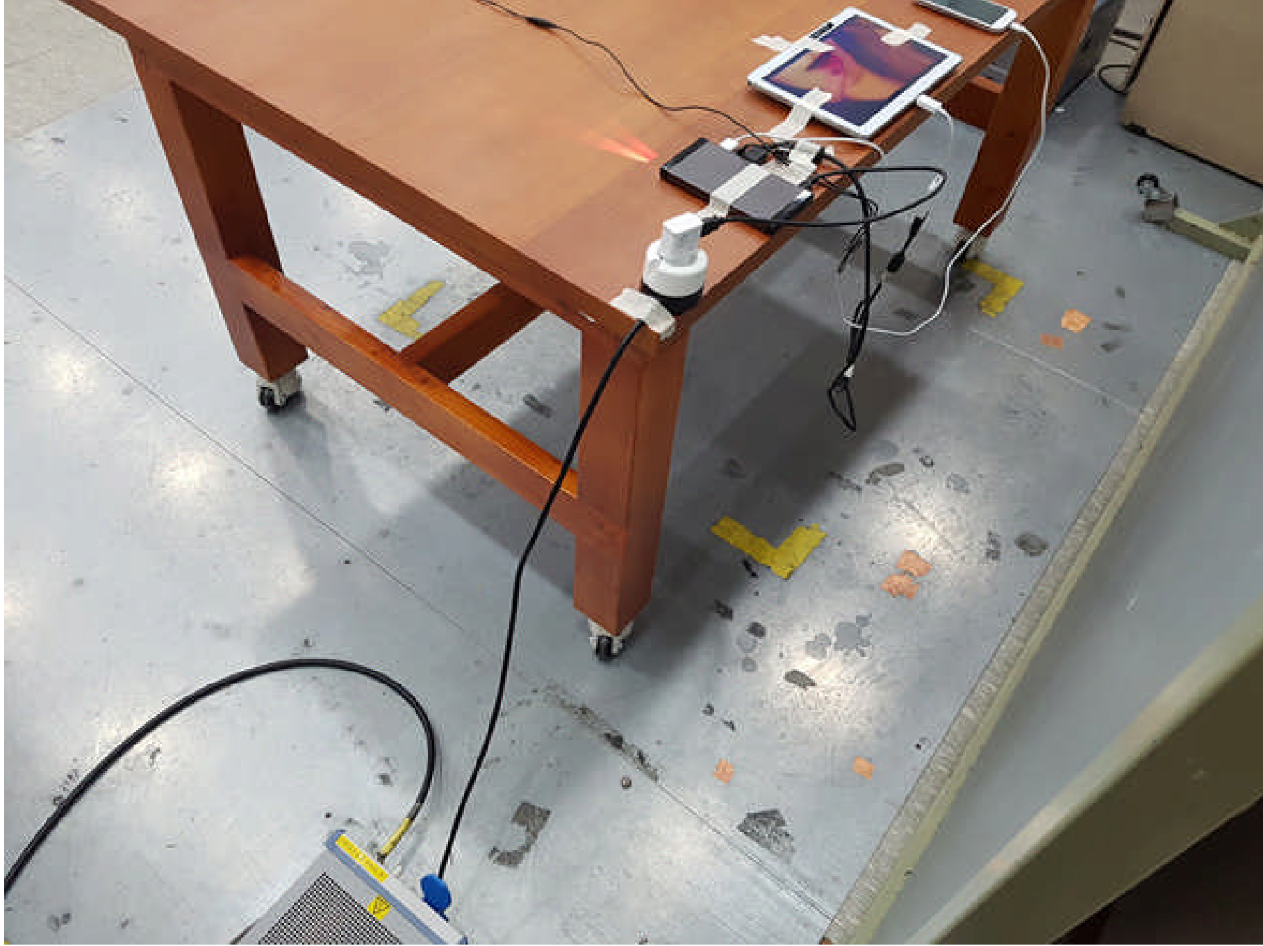
Conducted Emission _ Rear
