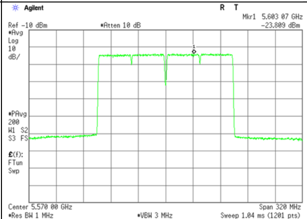
5570 MHz
