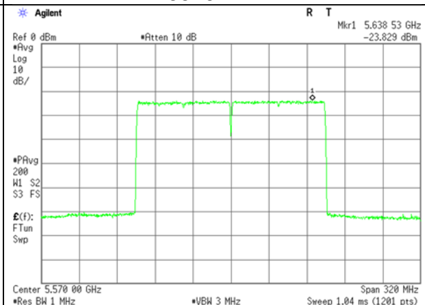
5570 MHz
