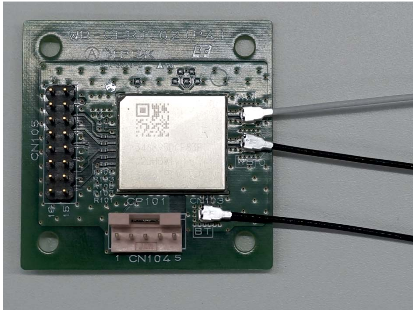
Module with Antenna (L34RF022, L34RF023, L34RF024)
