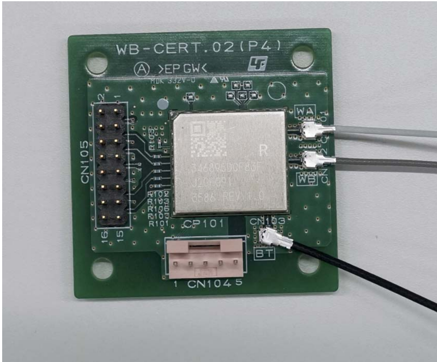
Module with Antenna (2299057-3, 2299057-2, 2299057-1)
