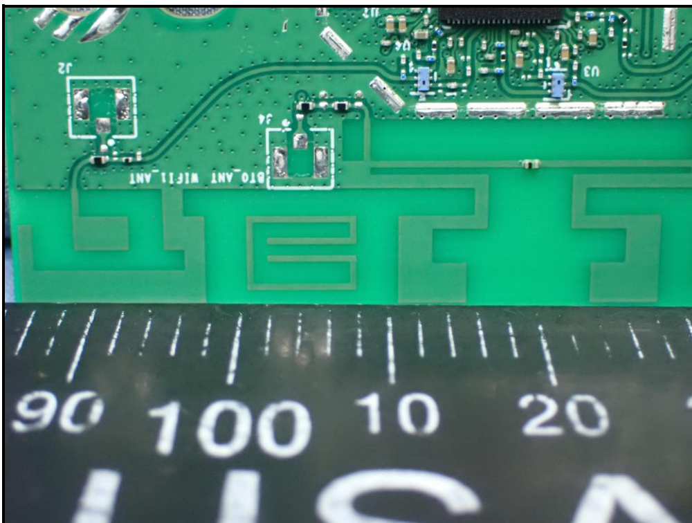
Antenna_BT 0
