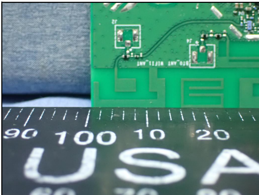
Antenna_Wifi 0
