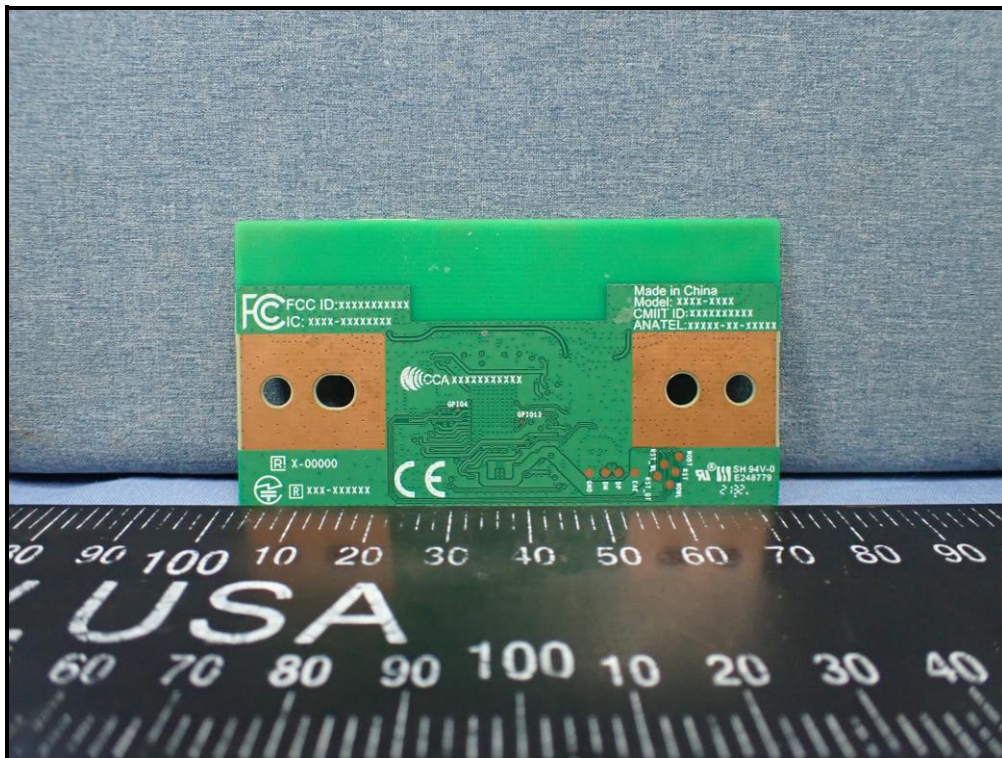
Antenna_Wifi 0
