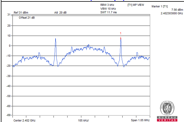
BT-LE Coded (125kbps) / CH 0
