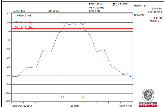
BT-LE Coded (125kbps) / CH 0
