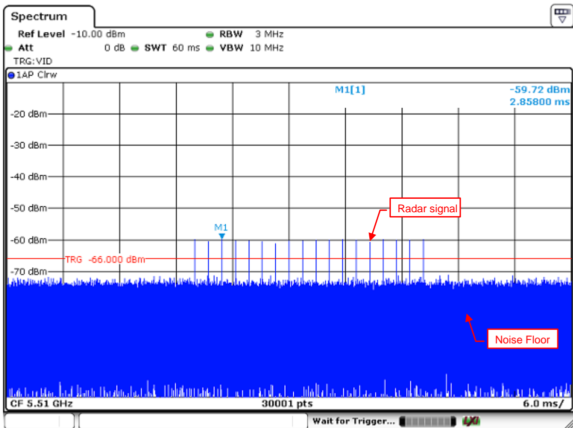
Radar Signal 0
