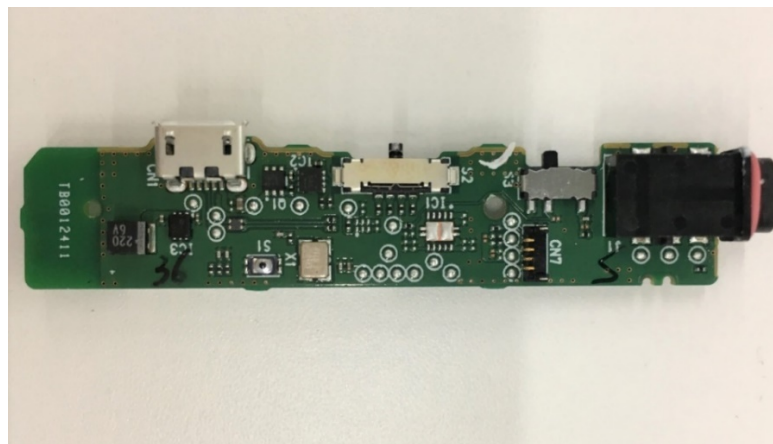
Main PWB (back-side)
