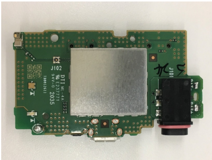
Main PWB surface
