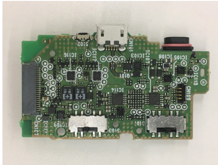
Main PWB back-side
