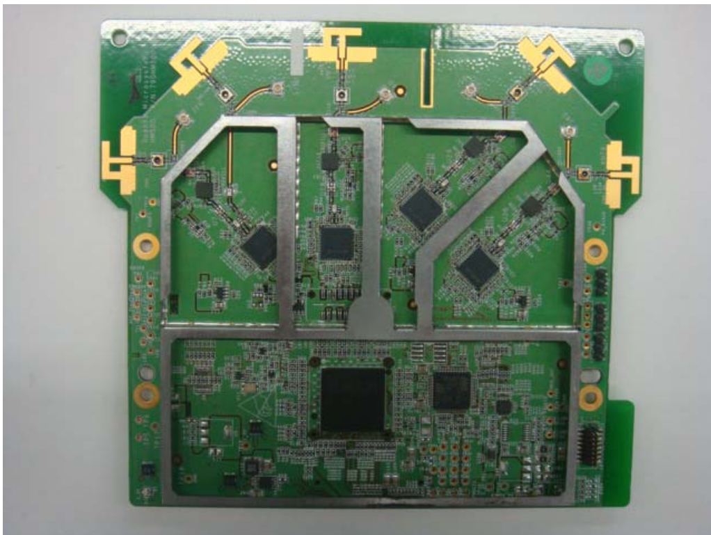
WHDI module Top (without shield)
