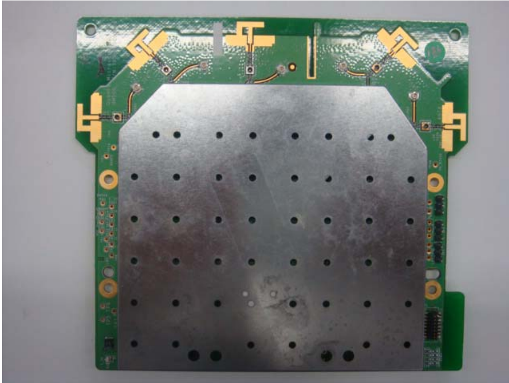
WHDI module Top (with shield)
