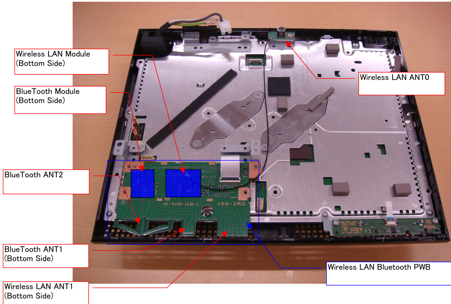
Photo. 1-2 Layout of WLAN_BT Module and Antenna (Without AC/DC PS Unit, Drive and Shield of WLAN_BT PWB)
