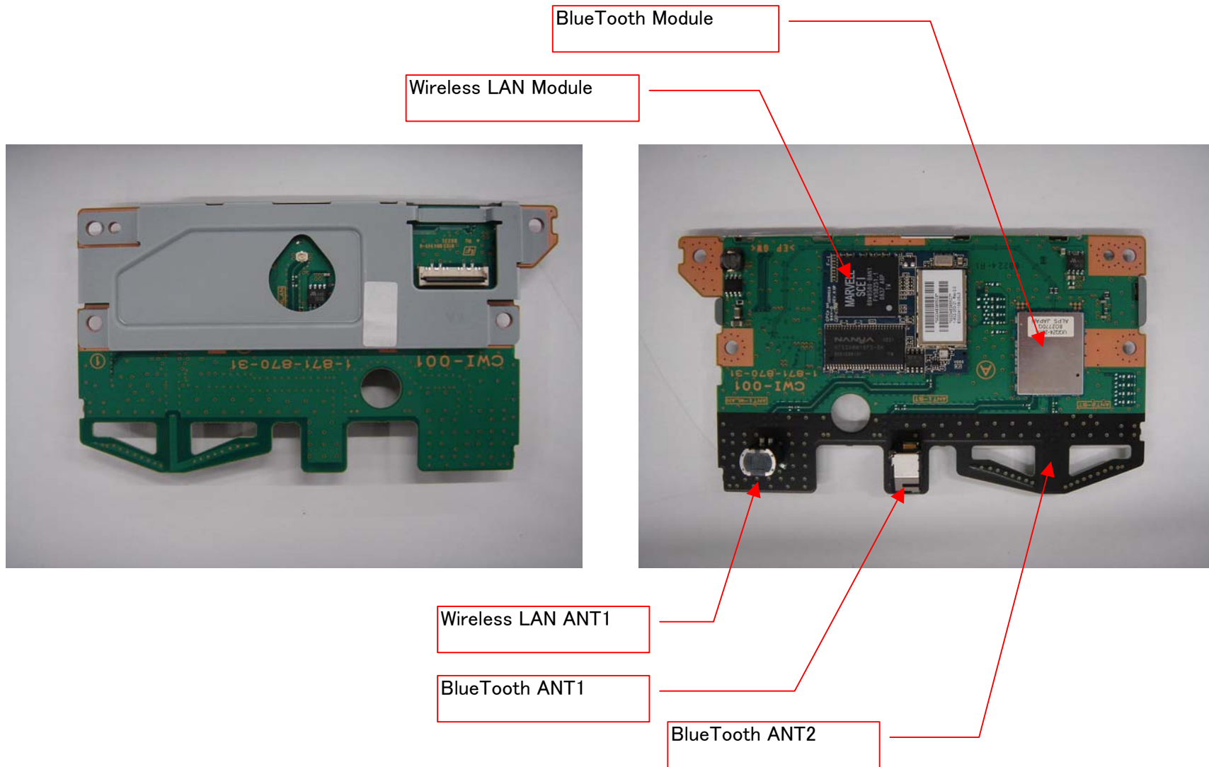
Photo. 2 WLAN_BT PWB (Module, Wireless LAN ANT1, BlueTooth ANT1, BlueTooth ANT2)
