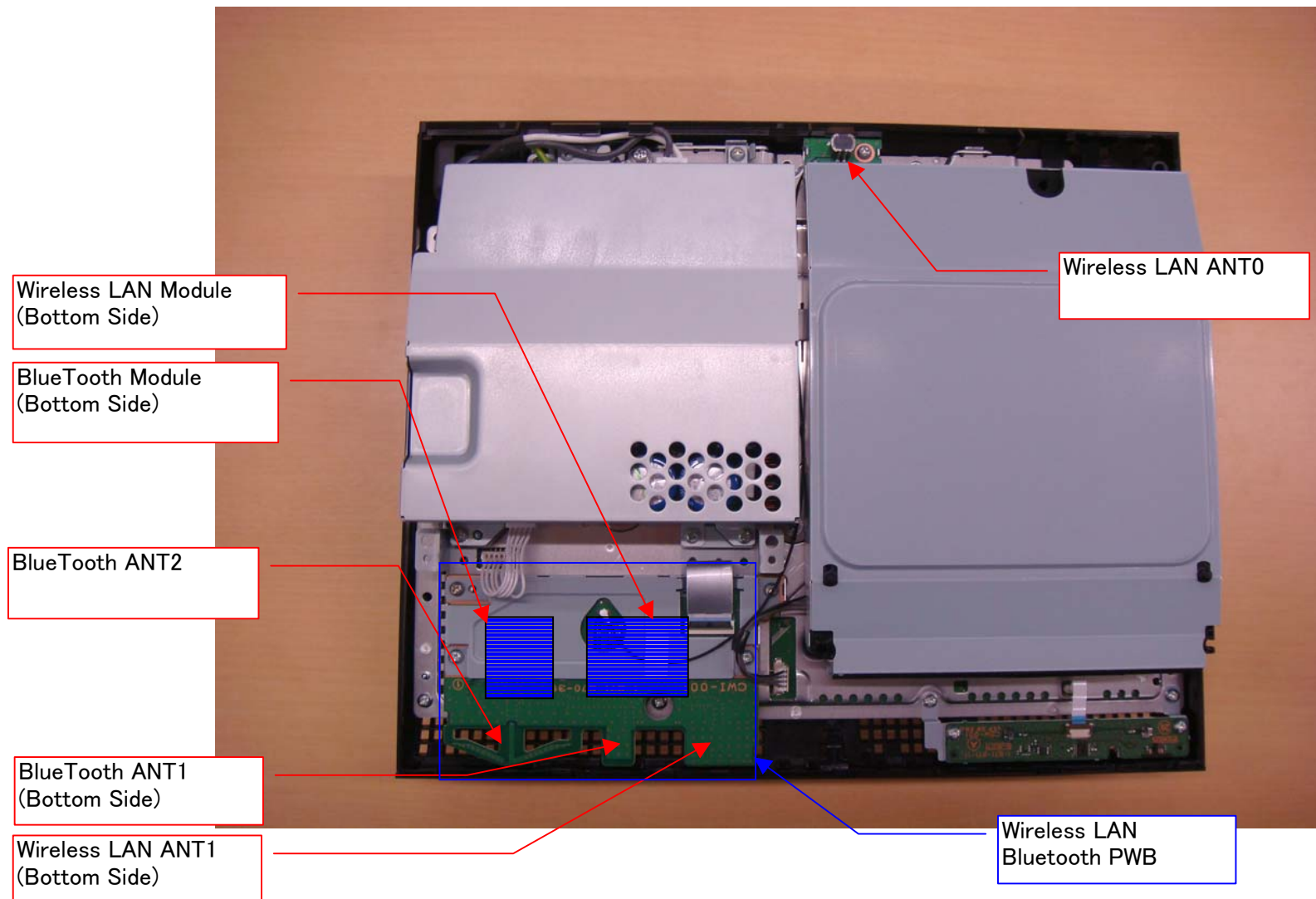
Photo. 1-1 Layout of WLAN_BT Module and Antenna
