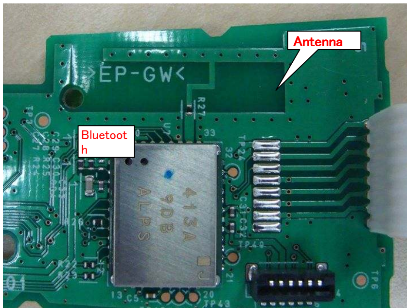
Photo 9 Inside(3/4) / Location of Antenna &Module
