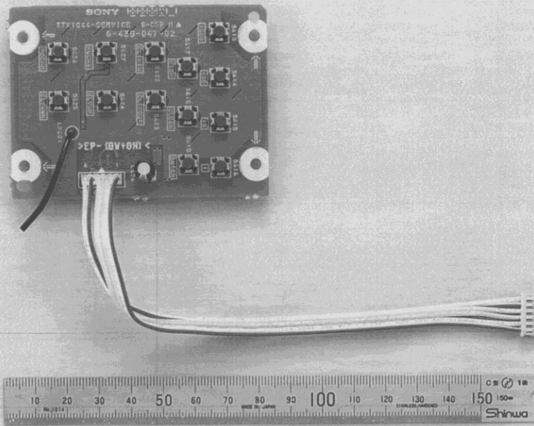
CDL1100-40 : SERVICE P.C.Board, Side A View
