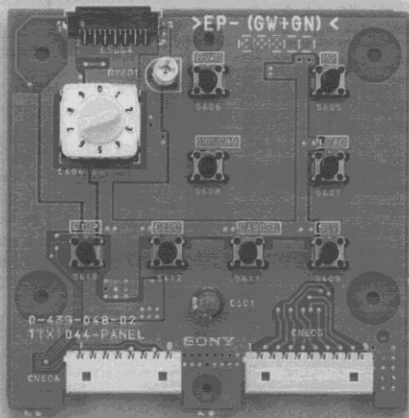
CDL1100-40 : PANEL SW P.C.Board, Side A View
