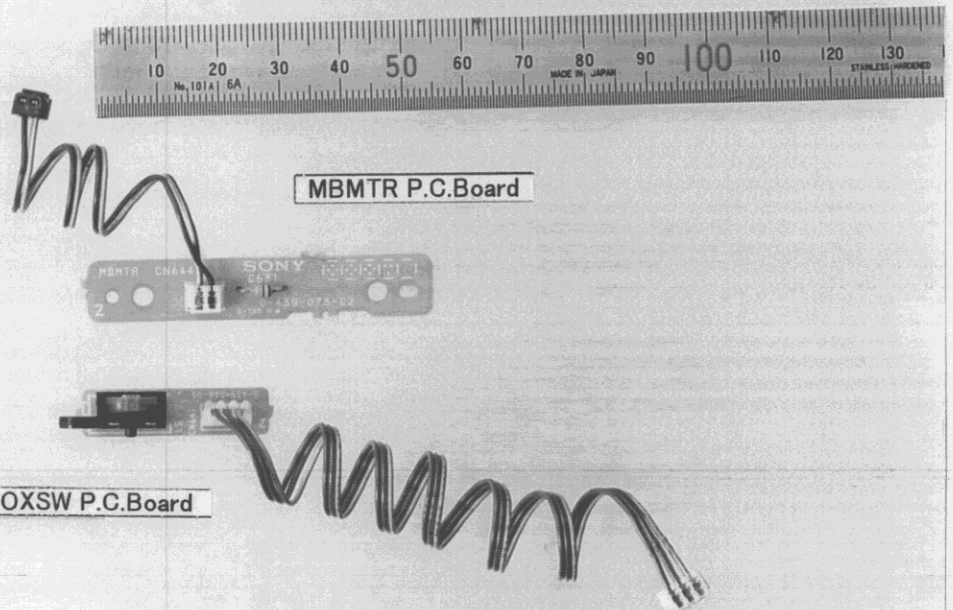
CDL1100-40 : Side A View
