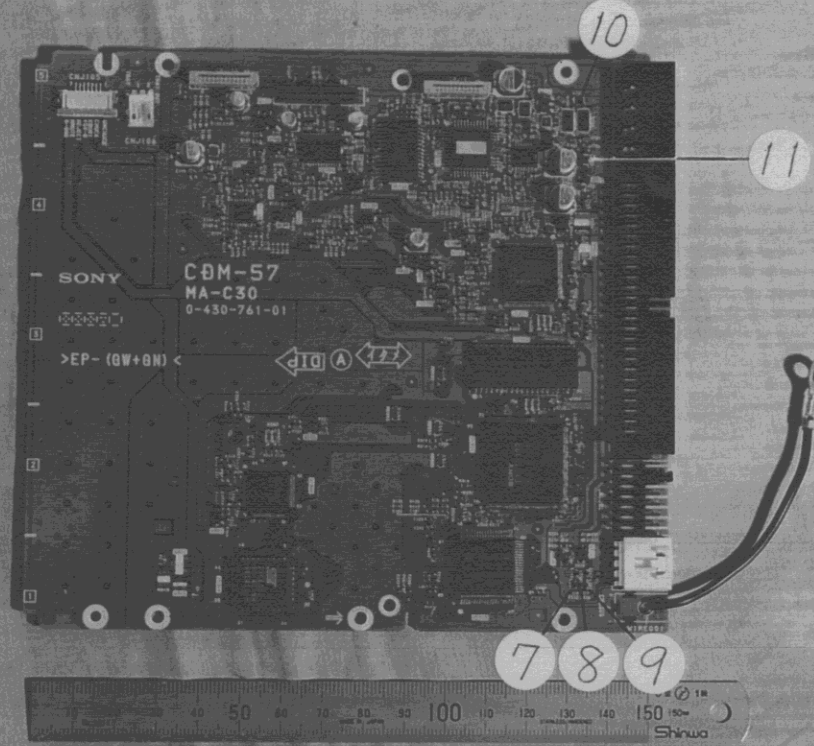
CDL1100-40 : CDM-57(CD-ROM DRIVE UNIT) ; MA-C30 P.C.Board, Side A View
