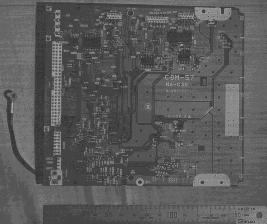
CDL1100-40 : CDM-57(CD-ROM DRIVE UNIT) ; MA-C30 P.C.Board, Side B View
