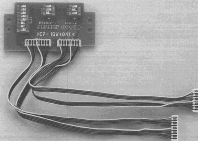
CDL1100-40 : DIP SW P.C.Board, Side A View
