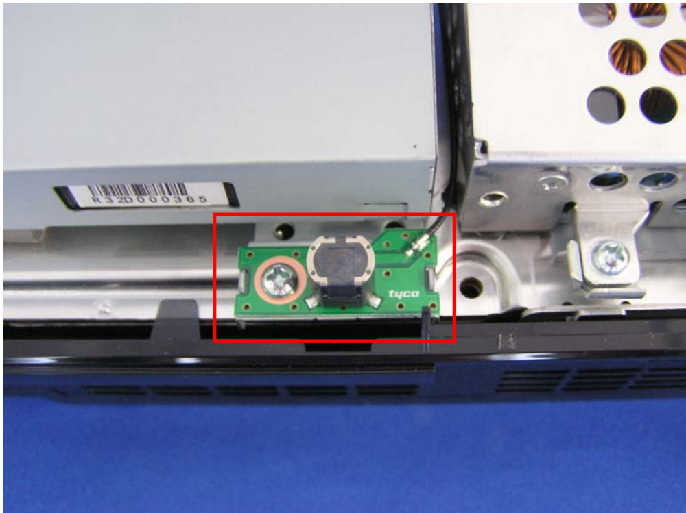
Close up Photo of WLAN Antenna-0
