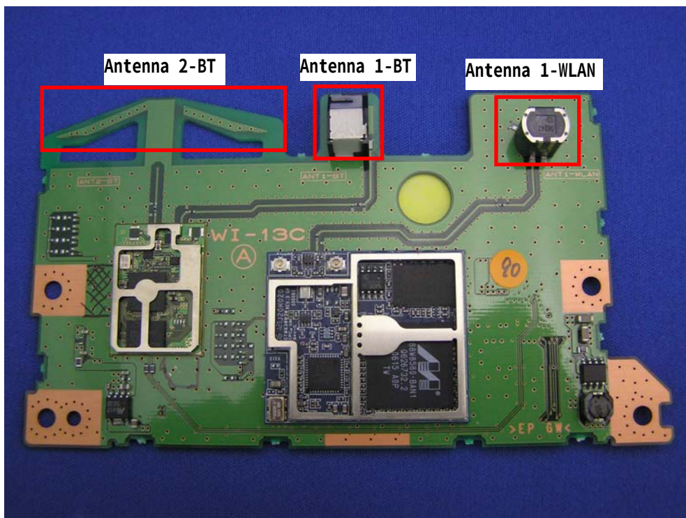
Top View of Board without shielding
