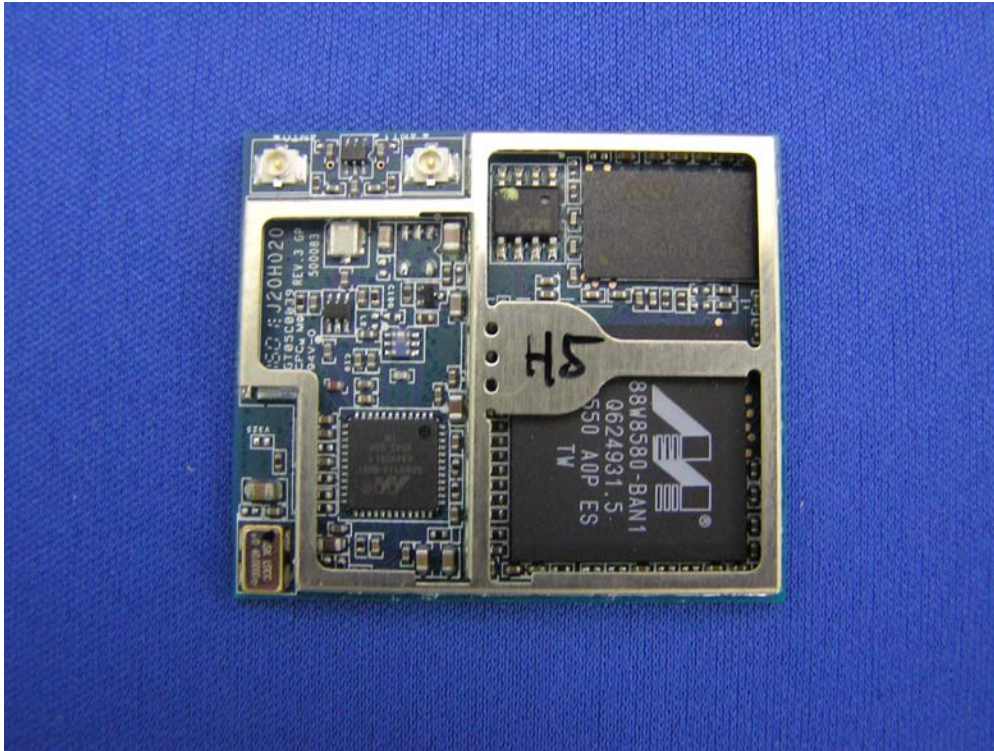
Top View of WLAN Module
