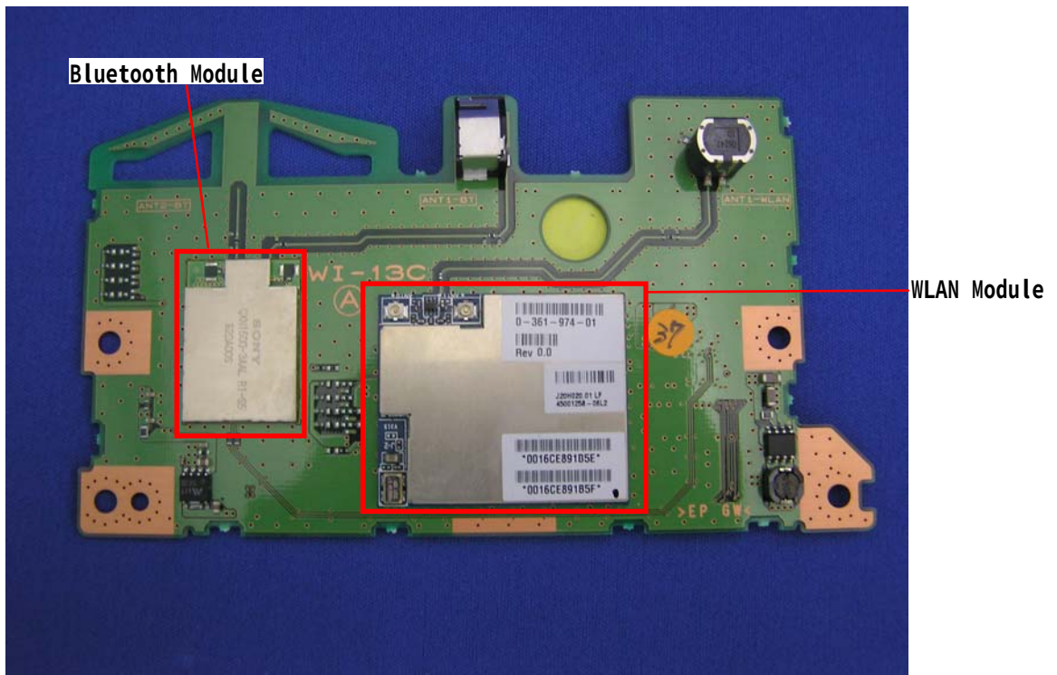
Top View of Board with shielding
