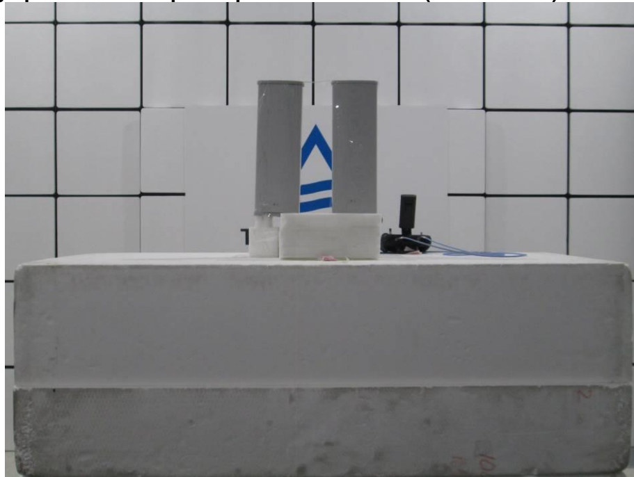
Photograph 8: Test Setup for Spurious Emissions (Front View 2)
