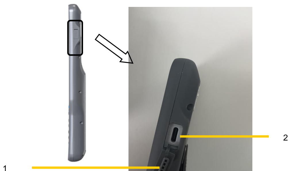
Figure 1-2-3 the port of SHC55
