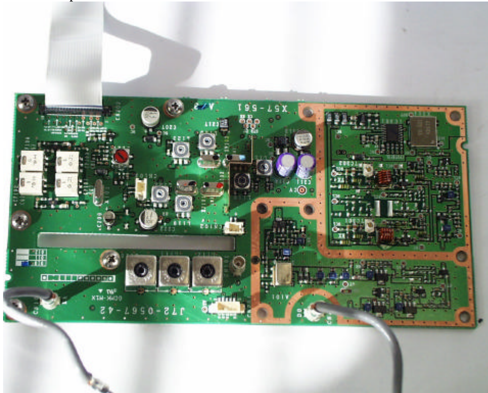
Transmitter printed circuit board.
