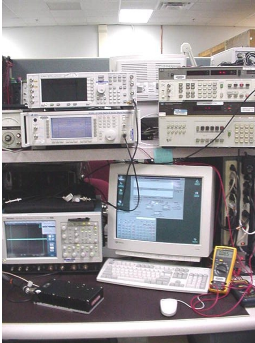
VDL Test Setup, Right Side equipment.
