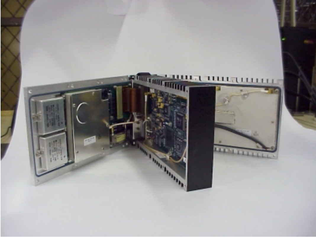
Exterior view showing the VDL-2000 open. The assembly on the left is the power supply. On the middle section, the circuit card visible is the DSP card. On the right is RF CCA, with its shield in place.
