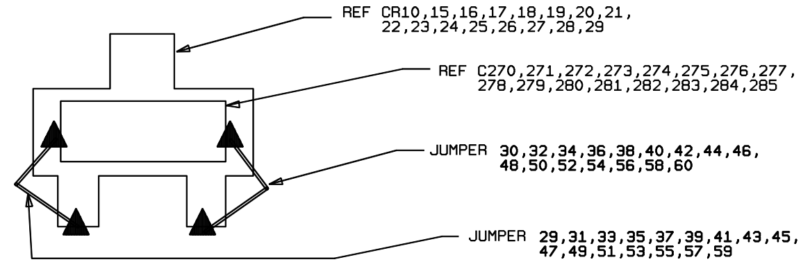
DETAIL H (FOR TOP SIDE JUMPERS)
