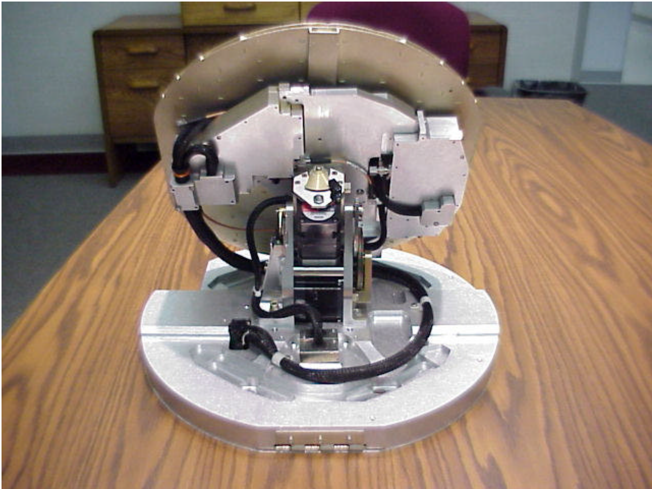
Figure 14. RTA-XXX Back - Left Side.
