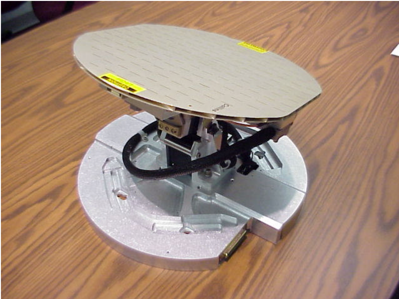
Figure 13. RTA-XXX Receiver/Transmitter Antenna.
